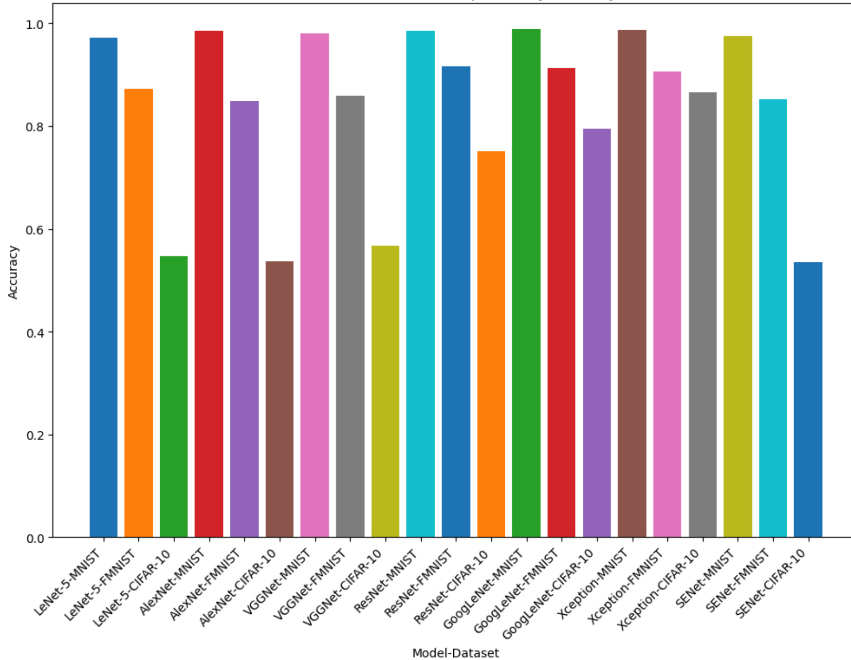
Model Performance Comparison by Accuracy
